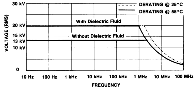
Fig. 1-2. Maximum input voltage derating with frequency.
