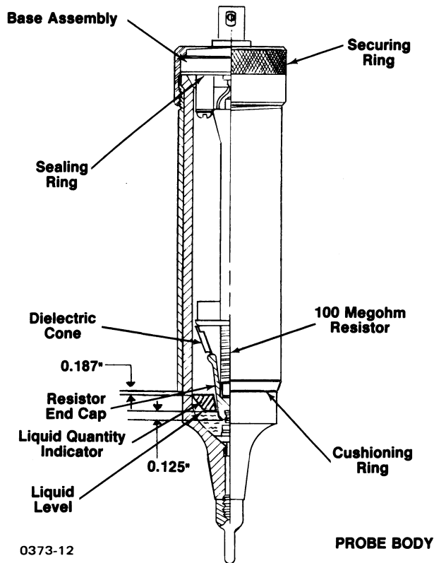
Fig. 4-1. Cutaway view of the P6015 Probe.
