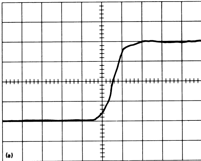
Fig. 2-2. Waveforms showing (a) Typical example of risetime within the probe's capability; and (b) example of risetime exceeding the probe's capability.
